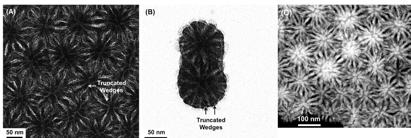
Figure 2. Top-view bright field TEM micrographs (A, B) and a top-view annular dark field scanning TEM micrograph (C) of mixed PtBA/PS brush-grafted 67 nm silica nanoparticles with PtBA M_n of 22.2 kDa and PS M_n of 23.4 kDa (MB-67-II) after being cast from \text{CHCl}_3 and annealed with \text{CHCl}_3 vapor for at least 3 h. The sample was stained at room temperature with \text{RuO}_4 vapor for 20 min.
