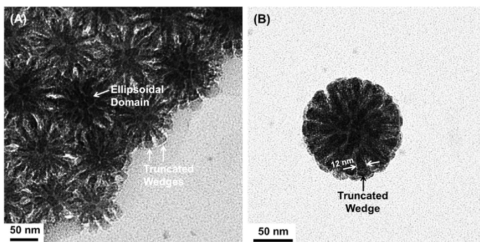
Figure 1. Top-view bright field TEM micrographs of mixed PtBA/PS brush-grafted 67 nm silica nanoparticles with PtBA M_n of 22.2 kDa and PS M_n of 18.7 kDa (MB-67-I) after being cast from \text{CHCl}_3 and annealed with \text{CHCl}_3 vapor for at least 3 h. The sample was stained at room temperature with \text{RuO}_4 vapor for 20 min.
