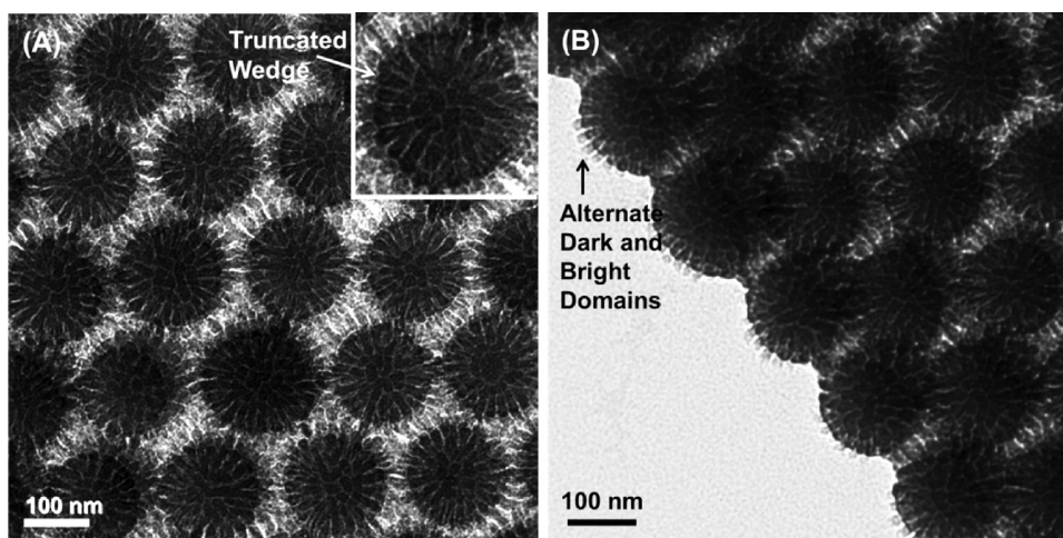
Figure 4. Top-view bright field TEM micrographs of mixed PtBA/PS brush-grafted 160 nm silica particles with PtBA M_n of 24.5 kDa and PS M_n of 18.7 kDa (MB-160) after being cast from \text{CHCl}_3 and annealed with \text{CHCl}_3 vapor for at least 3 h. The sample was stained at room temperature with \text{RuO}_4 vapor for 20 min.
